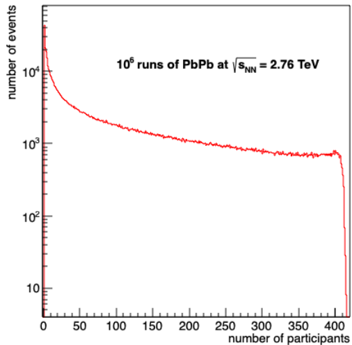
FIG. 8. Histogram of resulting N_{\text{part}} values.
