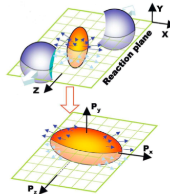
FIG. 2. Geometry of a non-central heavy ion collision.
