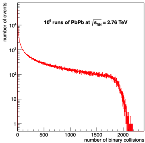
FIG. 9. Histogram of resulting N_{\text{coll}} values.
