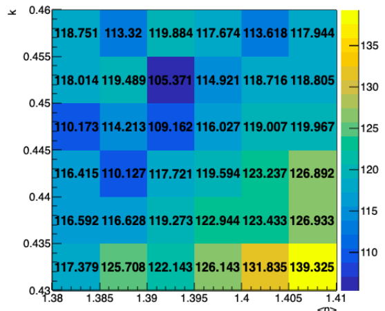
FIG. 11. Final scan of the \mu and k parameter space.
