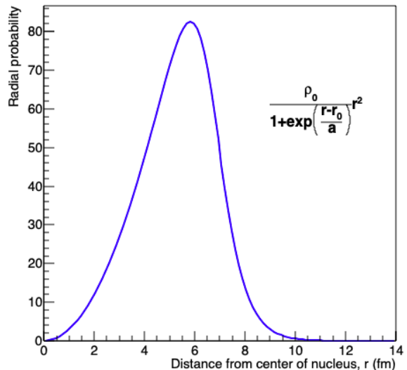
FIG. 5. Radial probability function for a Pb nucleus.
